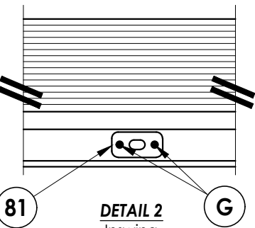
DETAIL 2 Inswing Standard Astragal Strike Plate @ Sill
