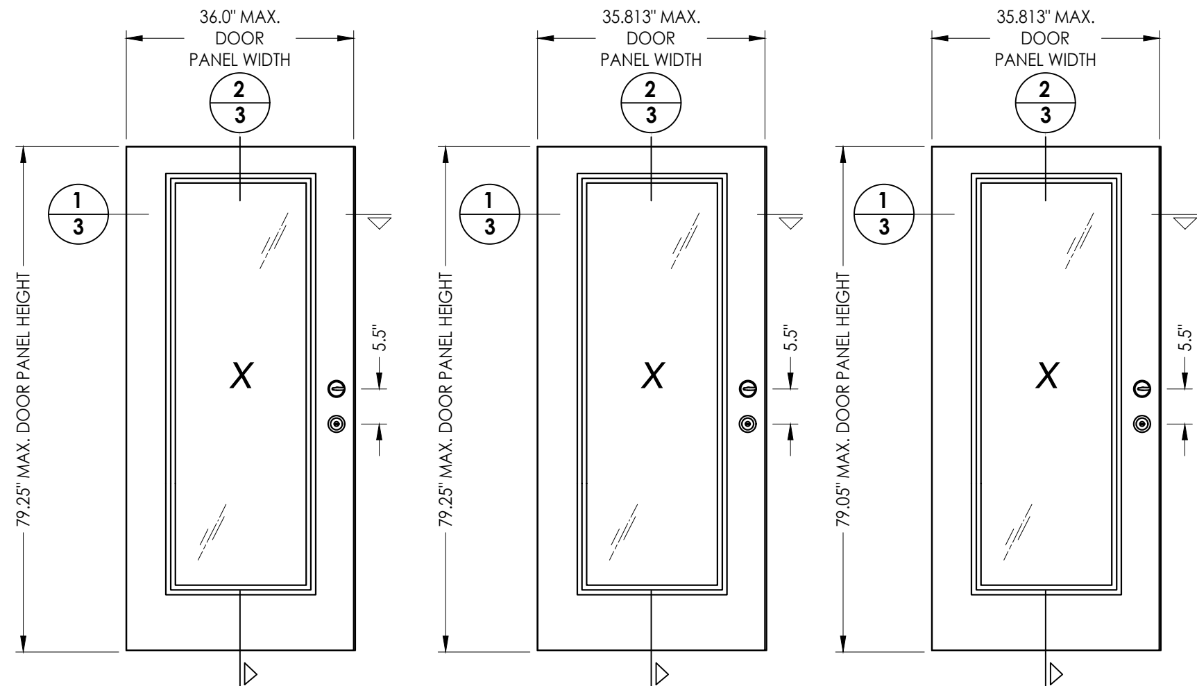
60 DOOR PANEL BOOK
