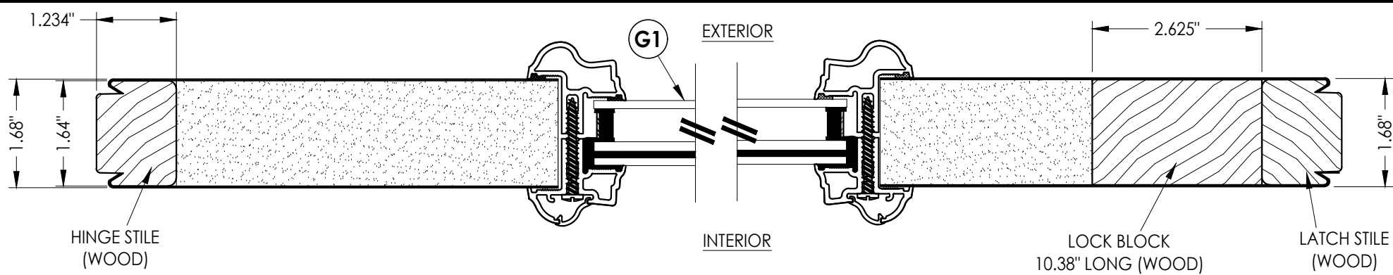
1 3 HORIZONTAL CROSS SECTION
